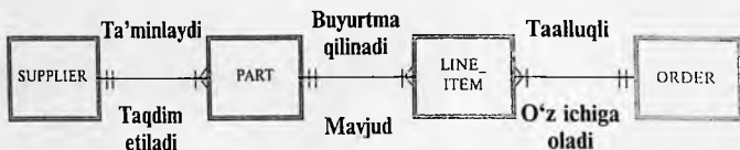
1.8.6-rasm. Shaxs-aloqa diagrammasi
