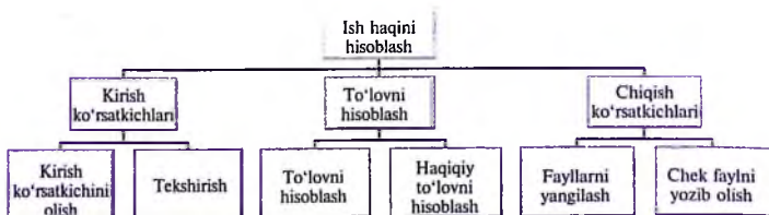
2.3.6-rasm. Ish haqini hisoblash tizimi tuzilmasi
