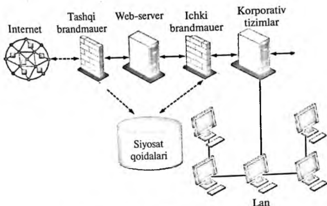
2.2.5-rasm. Korporativ brandmaueri
