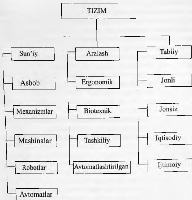
2.1.2-rasm. Tizimlar tasnifi
