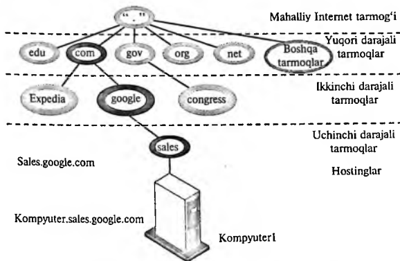
2.4.3-rasm. Domen nomlanish tizimi
