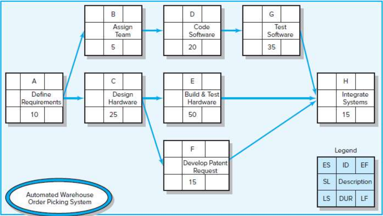
FIGURE 6.5 Activity-on-Node Network
