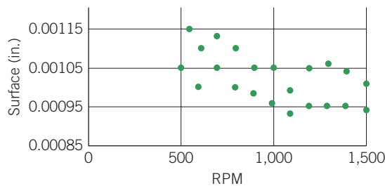
FIGURE 15.31 Scatter Diagram: Surface Flatness Versus Revolutions per Minute.
