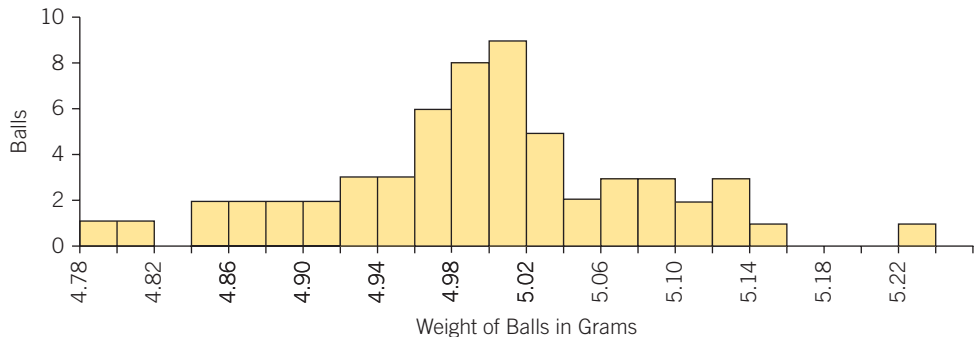
FIGURE 15.20 Histogram with Limited Amount of Data Stretched.
