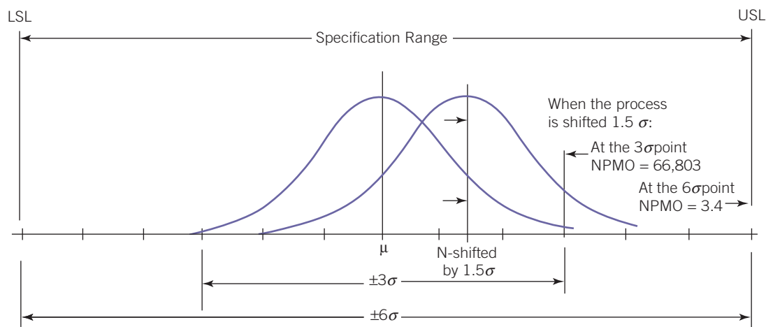
FIGURE 19.17 The 1½ Sigma Shift.
