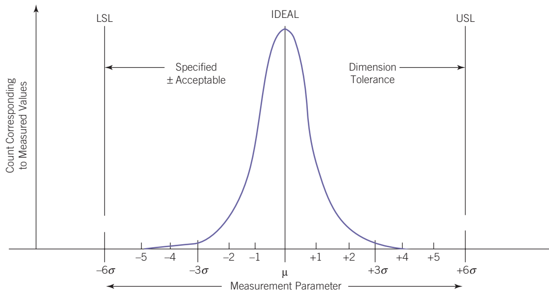
FIGURE 19.14 Histogram of a 6-Sigma Process.
