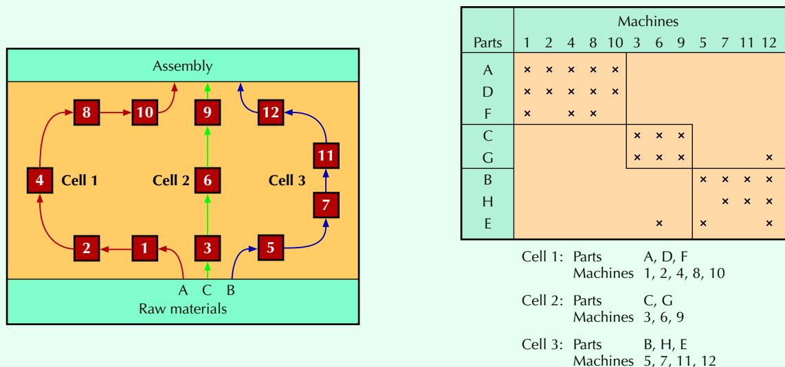
FIGURE 7.12 Revised Cellular Layout with Reordered Routing Matrix
