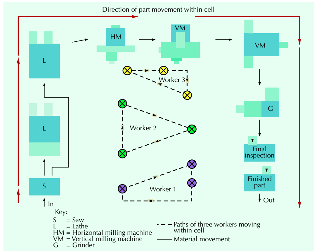
FIGURE 7.13 A Manufacturing Cell with Worker Paths
