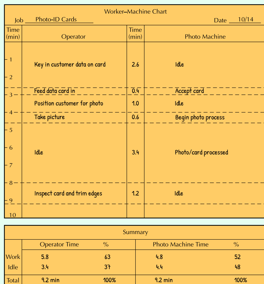
FIGURE 8.3 Worker-Machine Chart
