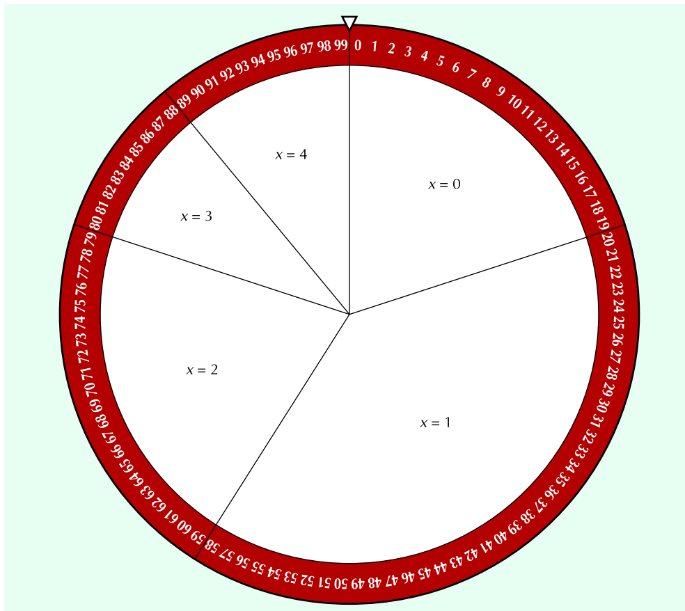
FIGURE S13.1 A Roulette Wheel of Demand
