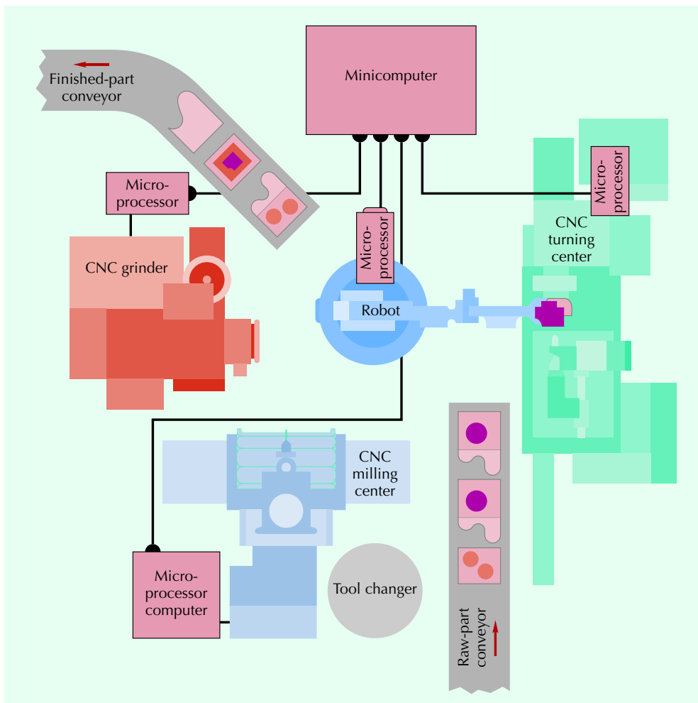
FIGURE 7.14 An Automated Manufacturing Cell
