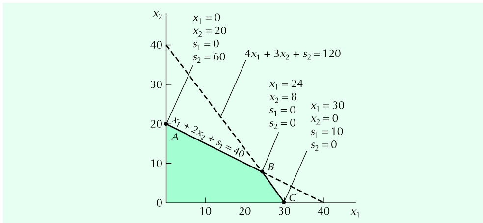
FIGURE S14.1 Solution Points with Slack Variables
