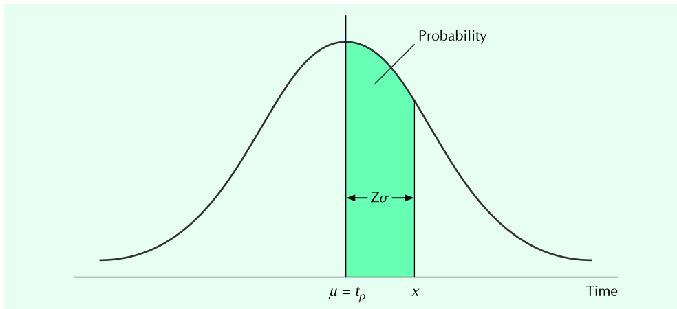
FIGURE 9.14 Normal Distribution of Project Time
