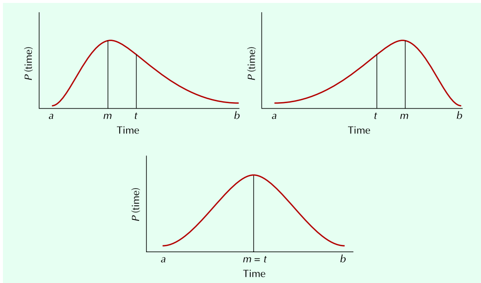
FIGURE 9.13 Examples of the Beta Distribution
