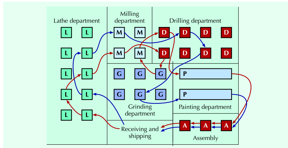
FIGURE 7.4 A Process Layout in Manufacturing
