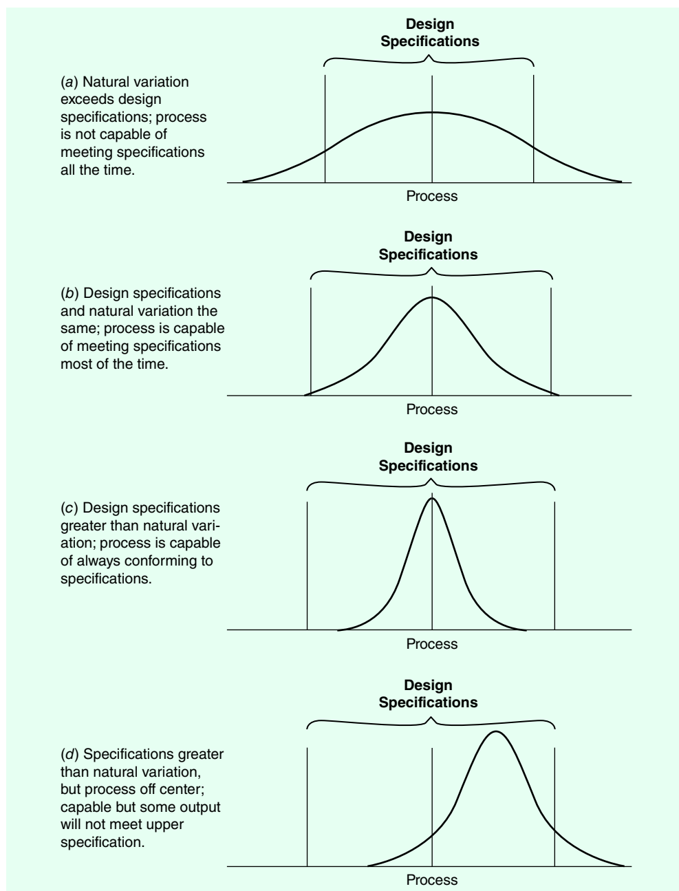
FIGURE 3.5 Process Capability
