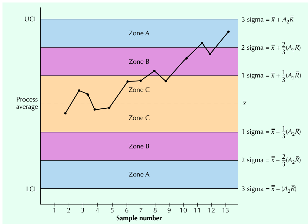
FIGURE 3.4 Zones for Pattern Tests
