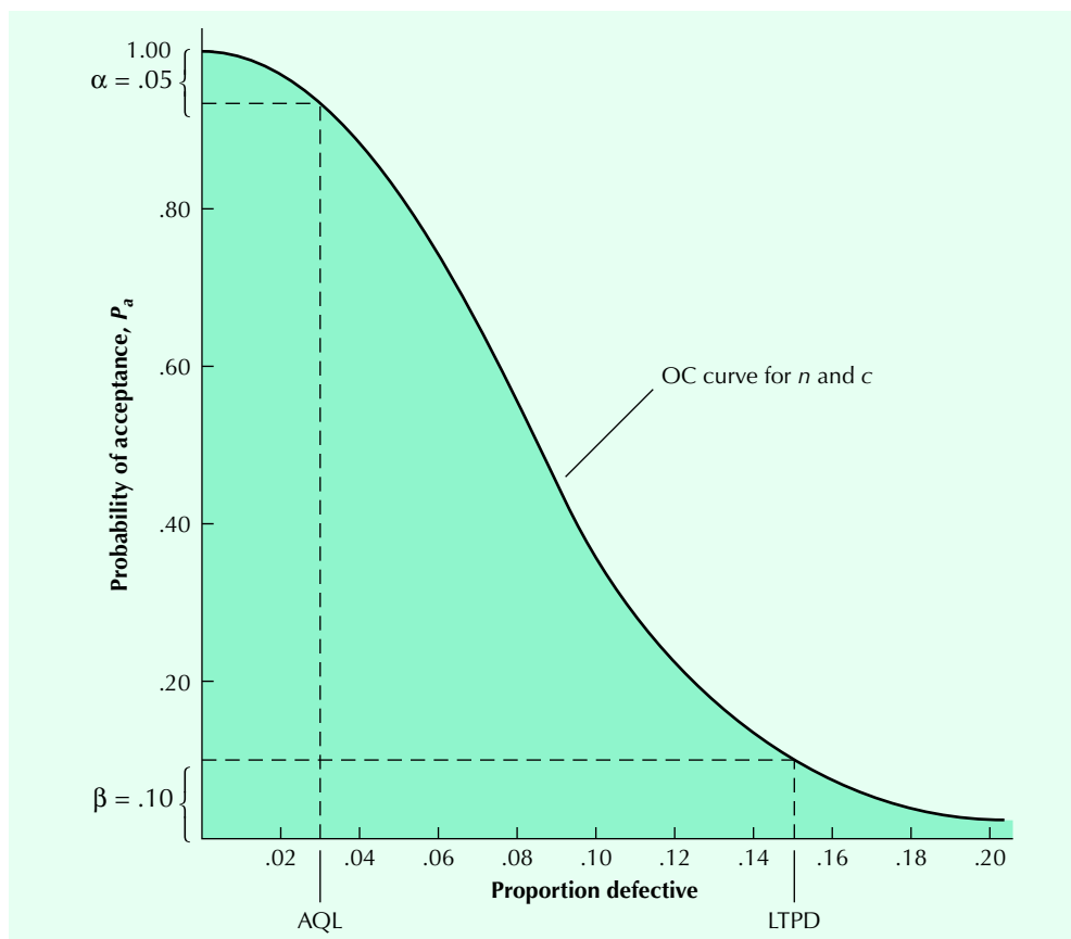
FIGURE S3.1 An Operating Characteristic Curve
