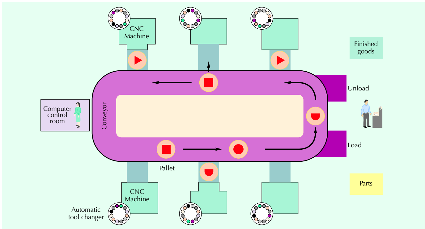
FIGURE 7.15 A Flexible Manufacturing System
