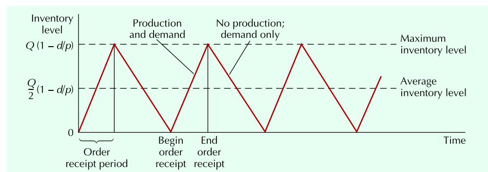
FIGURE 13.4 The Production Quantity Model
