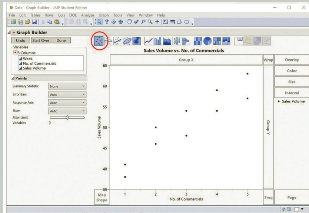
FIGURE JMP 2.4 Scatter Chart Created in JMP for the San Francisco Electronics Store Data
