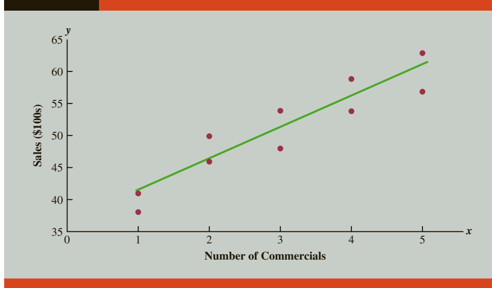
FIGURE 2.8 Scatter Diagram and Trendline for the San Francisco Electronics Store
