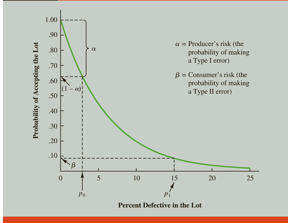
FIGURE 21.14 Operating Characteristic Curve for n = 15 , c = 0 with p_0 = .03 and p_1 = .15
