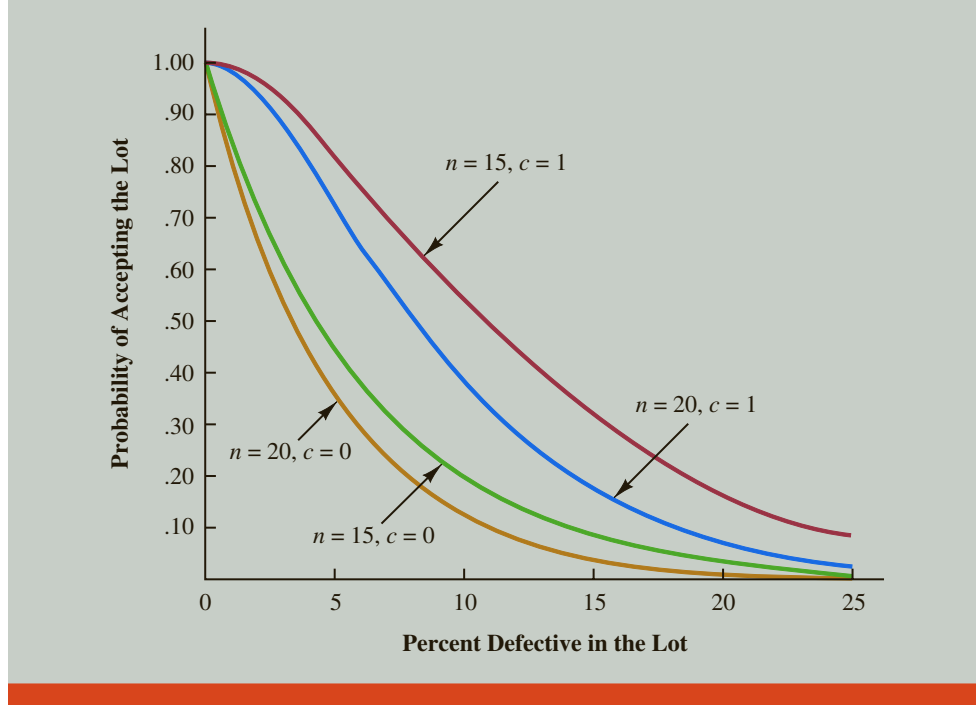
FIGURE 21.13 Operating Characteristic Curves for Four Acceptance Sampling Plans
