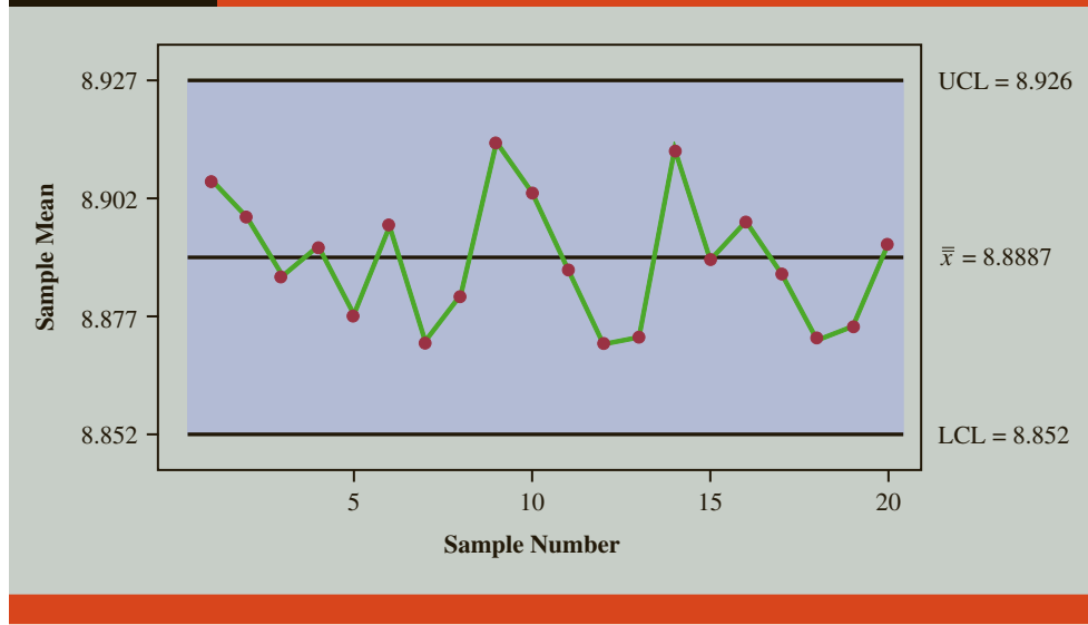
FIGURE 21.7 \bar{x} Chart for the Jensen Computer Supplies Problem
