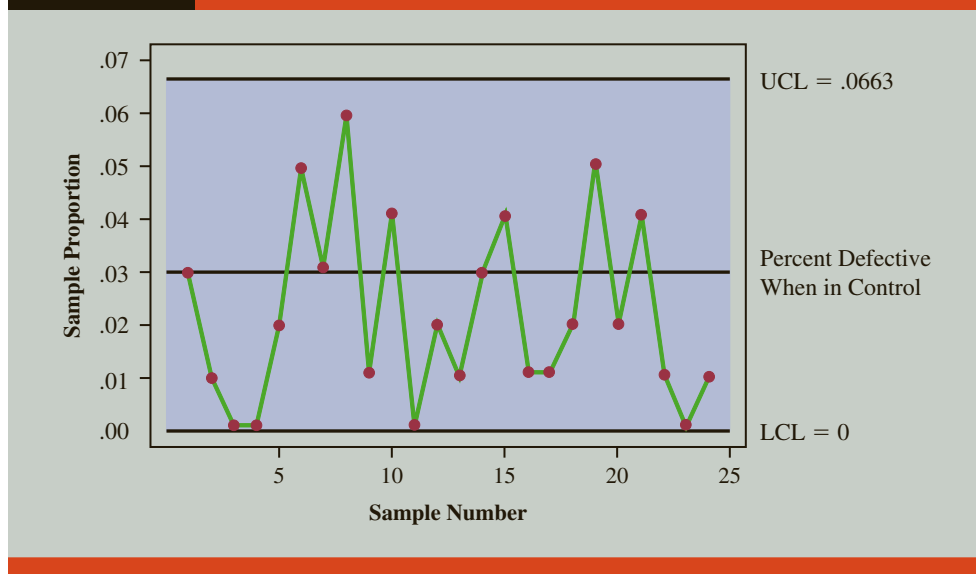
FIGURE 21.10 p Chart for the Proportion Defective in a Mail-Sorting Process
