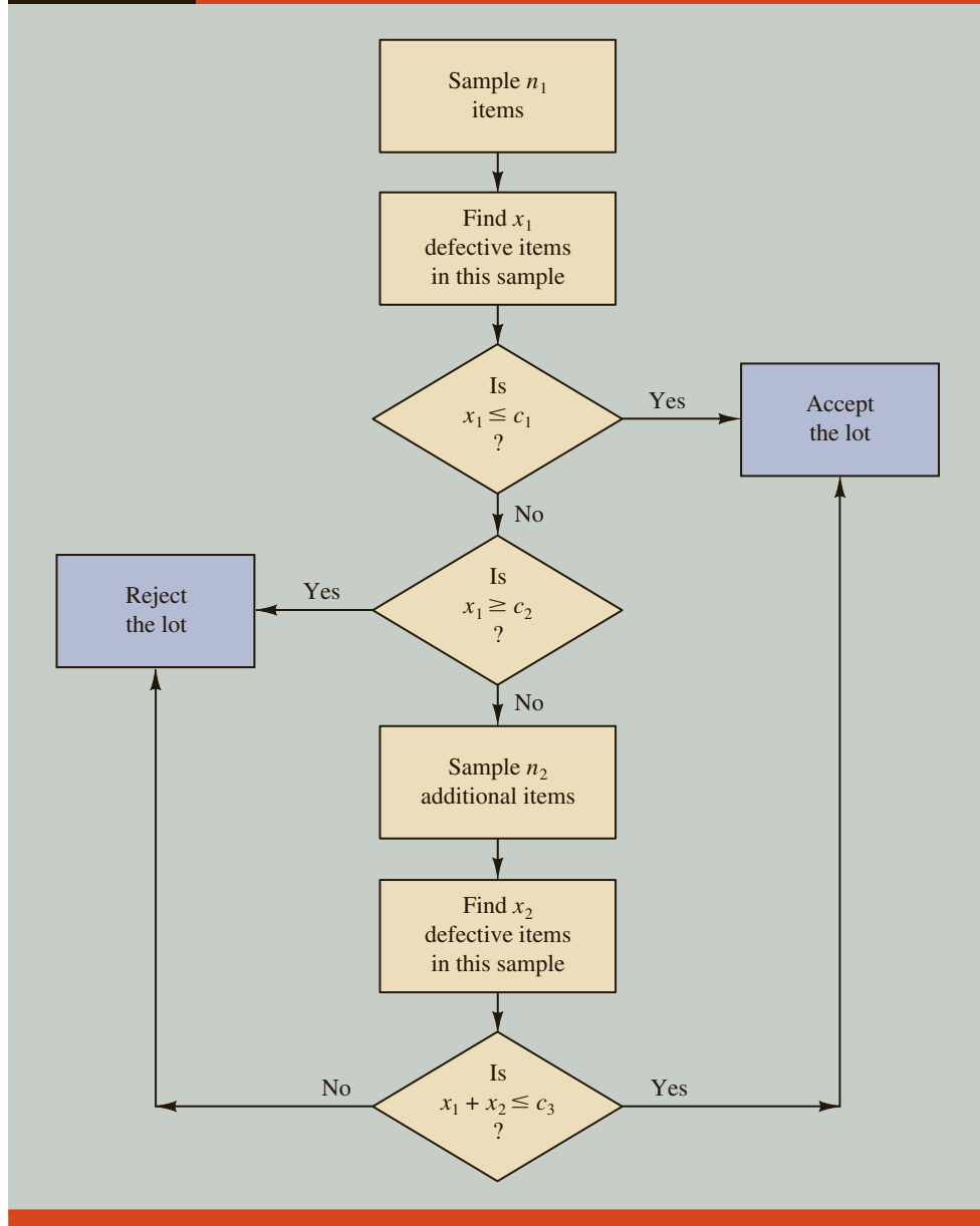
FIGURE 21.15 A Two-Stage Acceptance Sampling Plan
