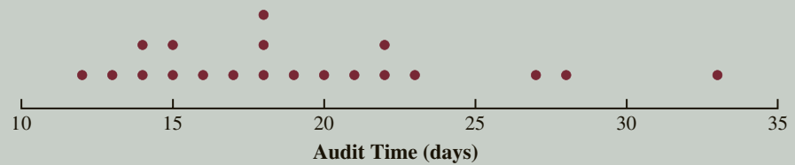
FIGURE 2.5 Dot Plot for the Audit Time Data
