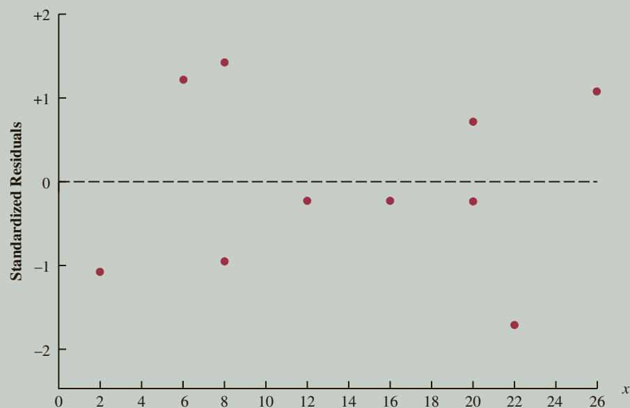
FIGURE 14.14 Plot of the Standardized Residuals Against the Independent Variable x for Armand's Pizza Parlors
