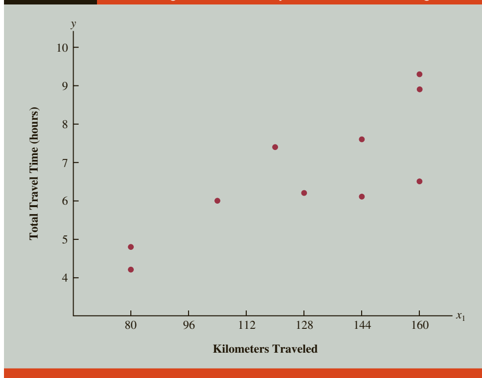
FIGURE 15.2 Scatter Diagram of Preliminary Data for Butler Trucking
