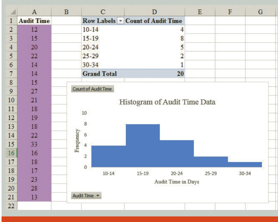
FIGURE Excel 2.3 Using Excel's PivotChart report to Construct a Frequency Distribution and Histogram for the Audit Time Data
