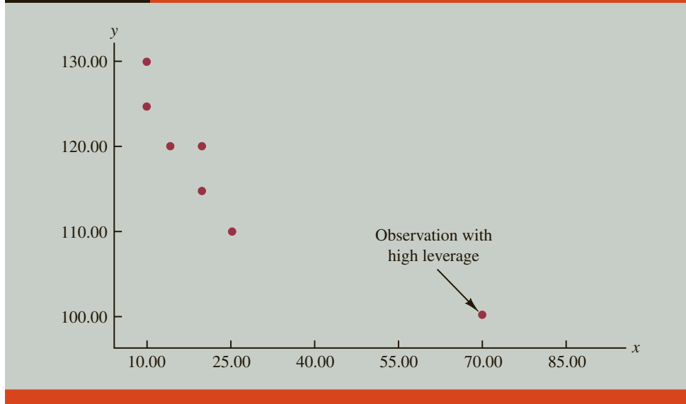
FIGURE 14.21 Scatter Diagram for the Data Set with a High Leverage Observation
