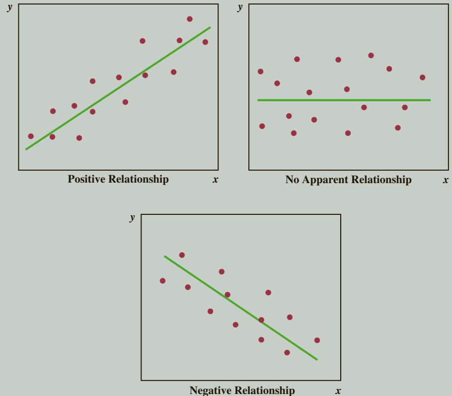
FIGURE 2.9 Types of Relationships Depicted by Scatter Diagrams
