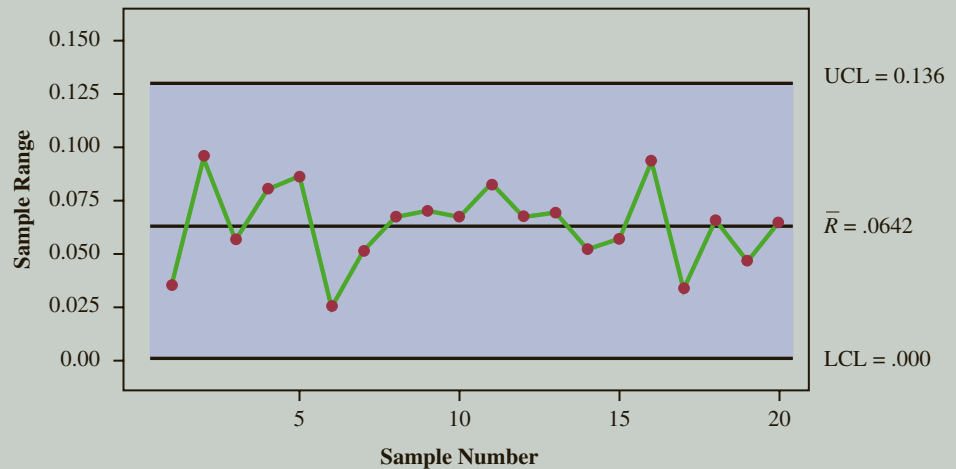
FIGURE 21.8 R Chart for the Jensen Computer Supplies Problem
