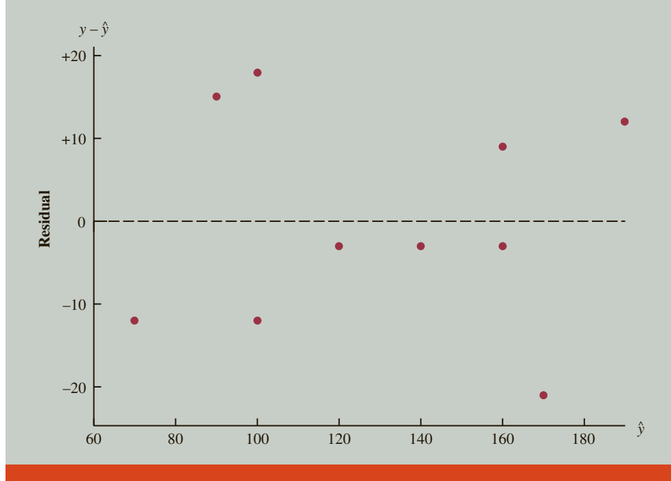
FIGURE 14.13 Plot of the Residuals Against the Predicted Values \hat{y} for Armand's Pizza Parlors
