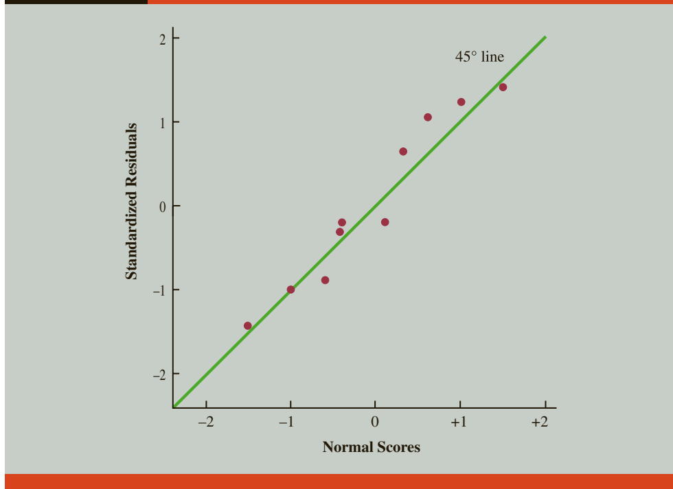
FIGURE 14.15 Normal Probability Plot for Armand's Pizza Parlors
