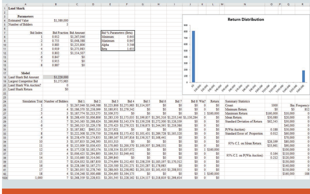
FIGURE 11.27 Output from Land Shark Simulation Using Beta Distribution for Bid Fraction Values
