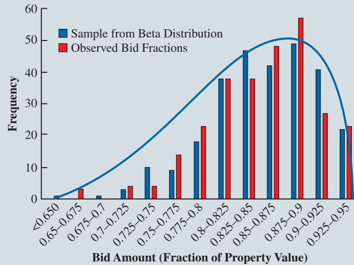
FIGURE 11.25 Fit of Beta Distribution to Bid Fraction Data
