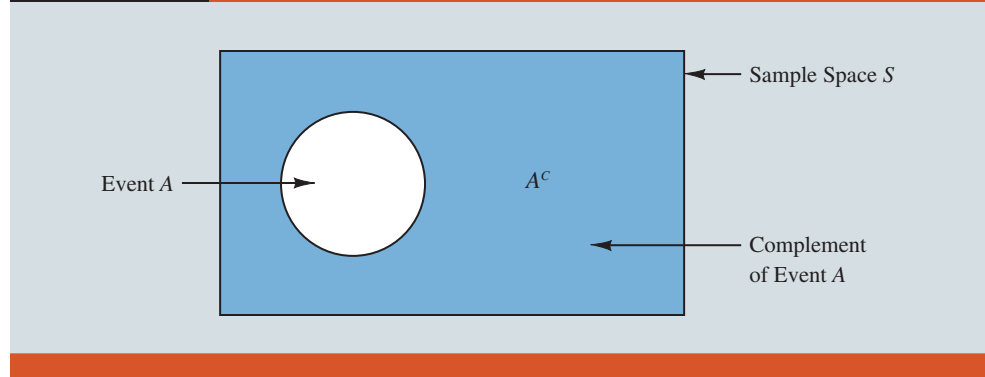
FIGURE 4.1 Venn Diagram for Event A
