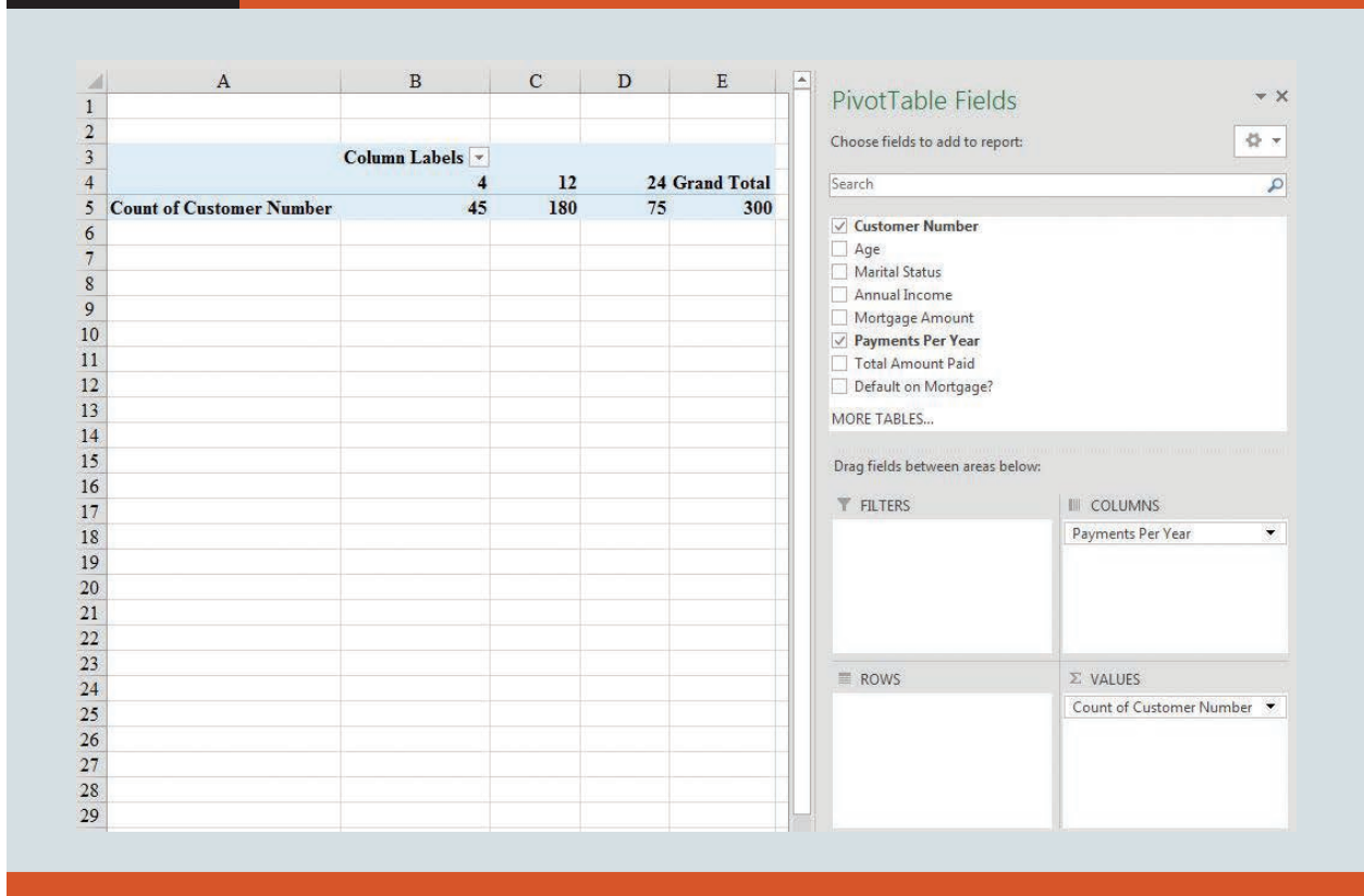
FIGURE 4.10 Excel PivotTable for Number of Payments Made per Year
