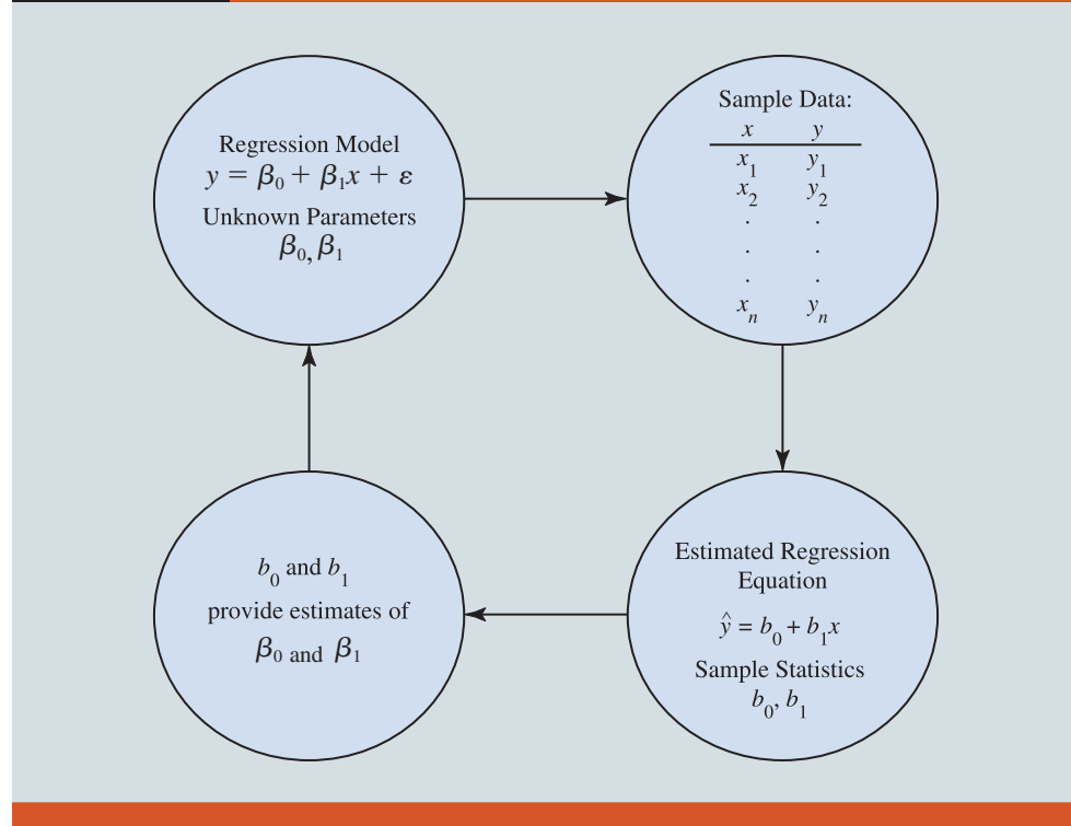
FIGURE 7.1 The Estimation Process in Simple Linear Regression
