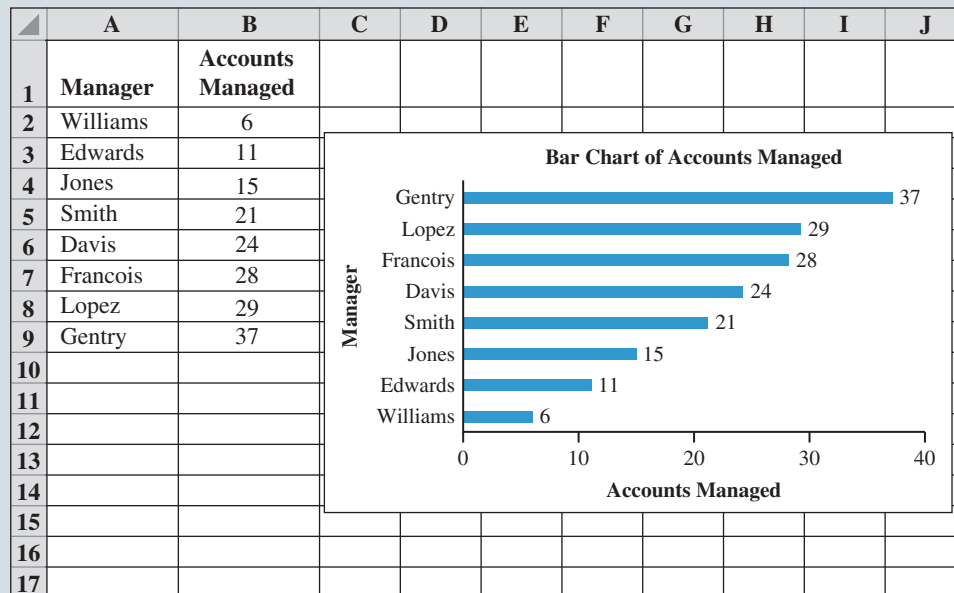
Bar Chart with Data Labels for Accounts Managed Data
