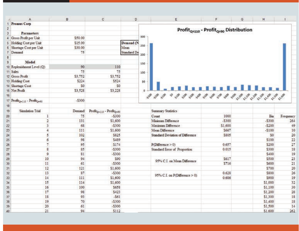
FIGURE 11.16 Output Worksheet for Promus Corp
