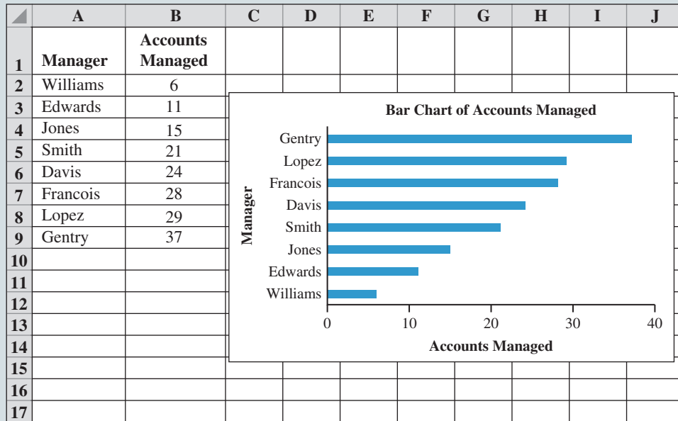
Sorted Bar Chart for Accounts Managed Data
