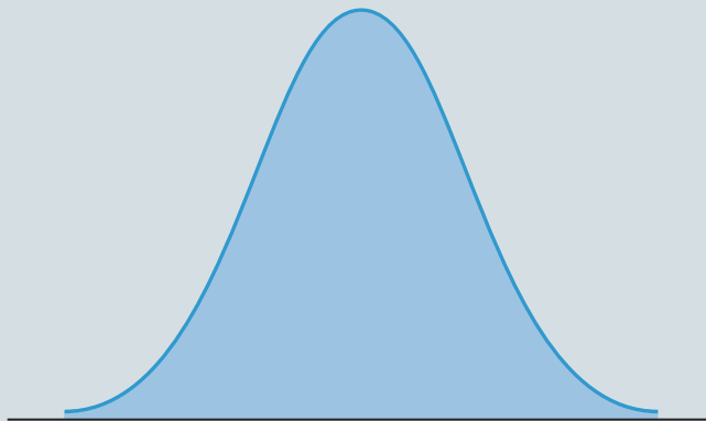
FIGURE 2.21 A Symmetric Bell-Shaped Distribution
