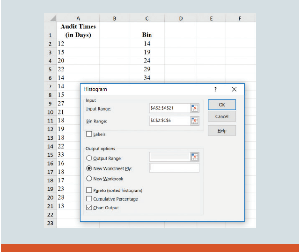
FIGURE 2.13 Creating a Histogram for the Audit Time Data Using Data Analysis ToolPak in Excel
