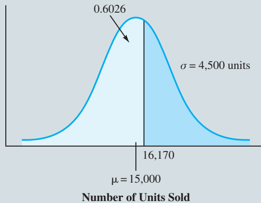
FIGURE 11.6 Generation of Value for First-Year Demand Corresponding to Random Number 0.6026
