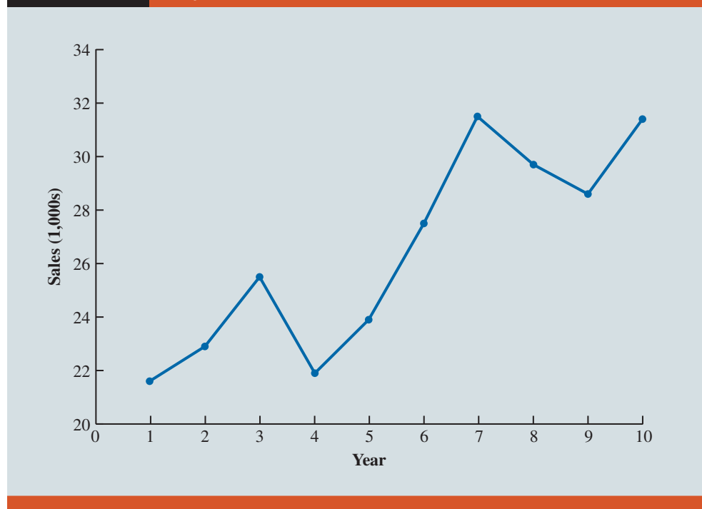
FIGURE 8.3 Bicycle Sales Time Series Plot
