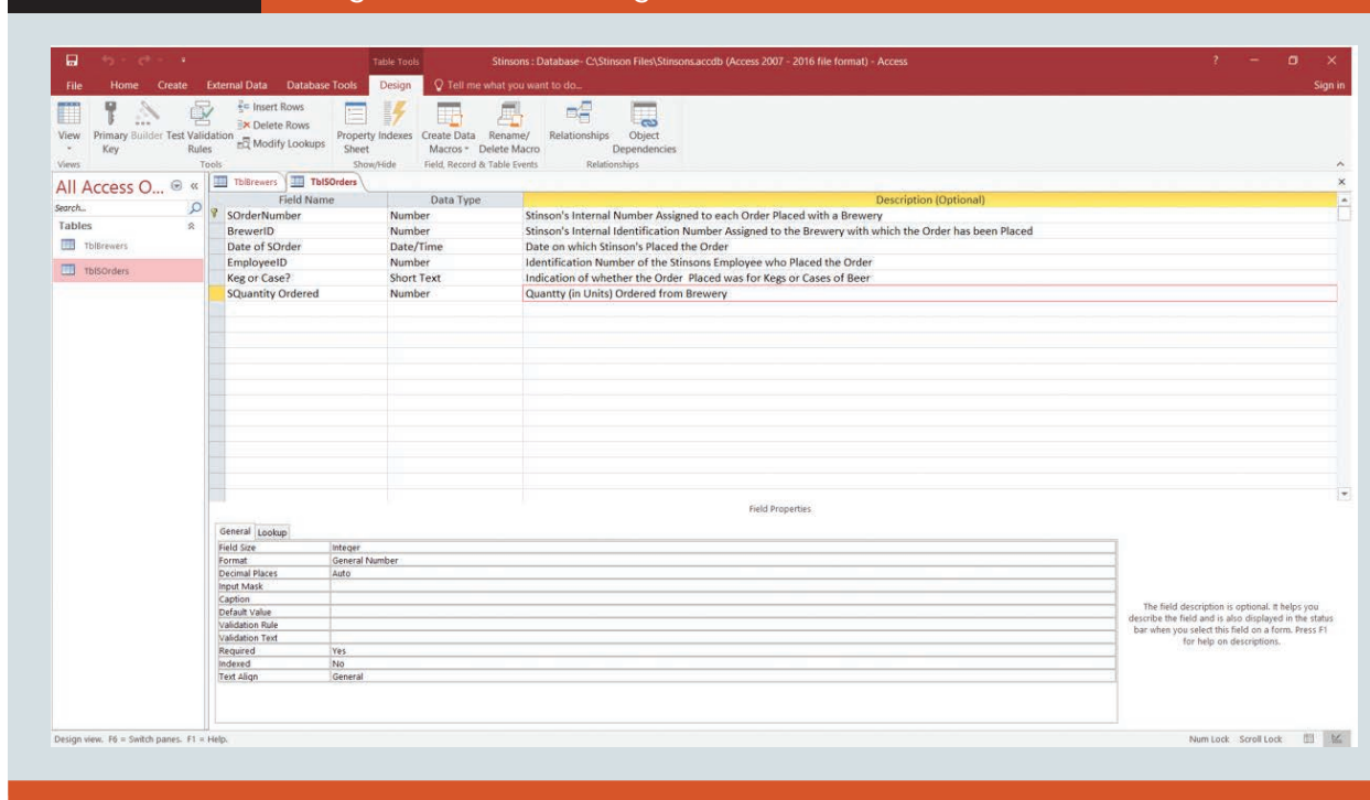
FIGURE B.11 Design View of Table Design for TbISOrders
