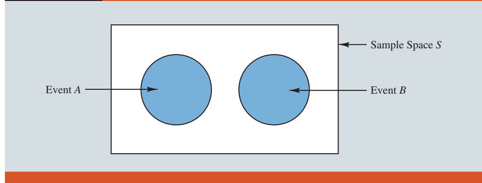
FIGURE 4.4 Venn Diagram for Mutually Exclusive Events
