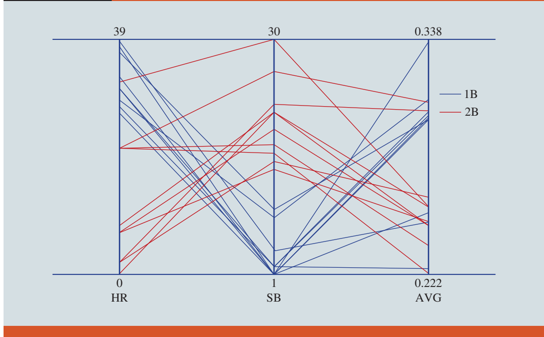
FIGURE 3.33 Parallel Coordinates Plot for Baseball Data
