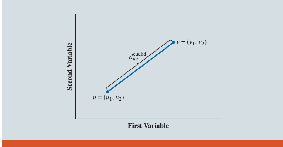
FIGURE 5.1 Euclidean Distance
