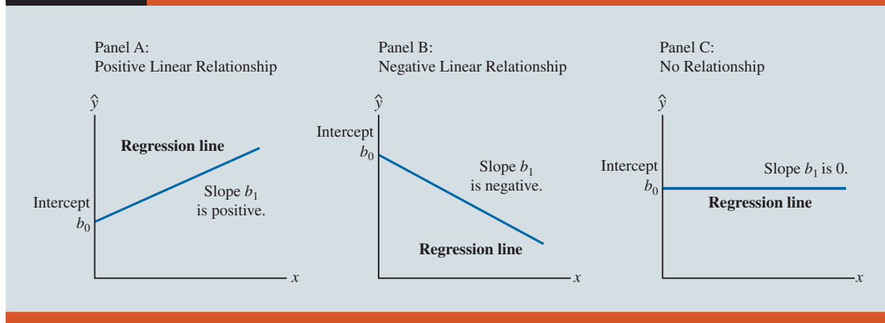
FIGURE 7.2 Possible Regression Lines in Simple Linear Regression
