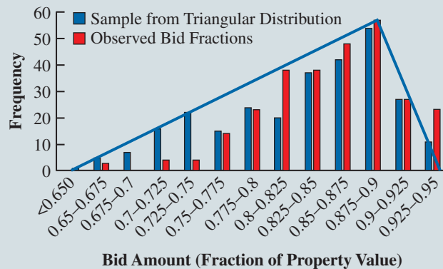
FIGURE 11.22 Fit of Triangular Distribution to Bid Fraction Data
