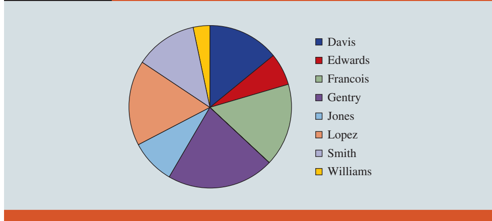
FIGURE 3.26 Pie Chart of Accounts Managed
