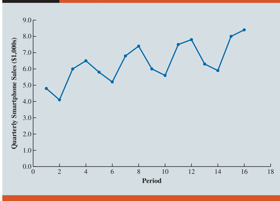
FIGURE 8.6 Quarterly Smartphone Sales Time Series Plot
