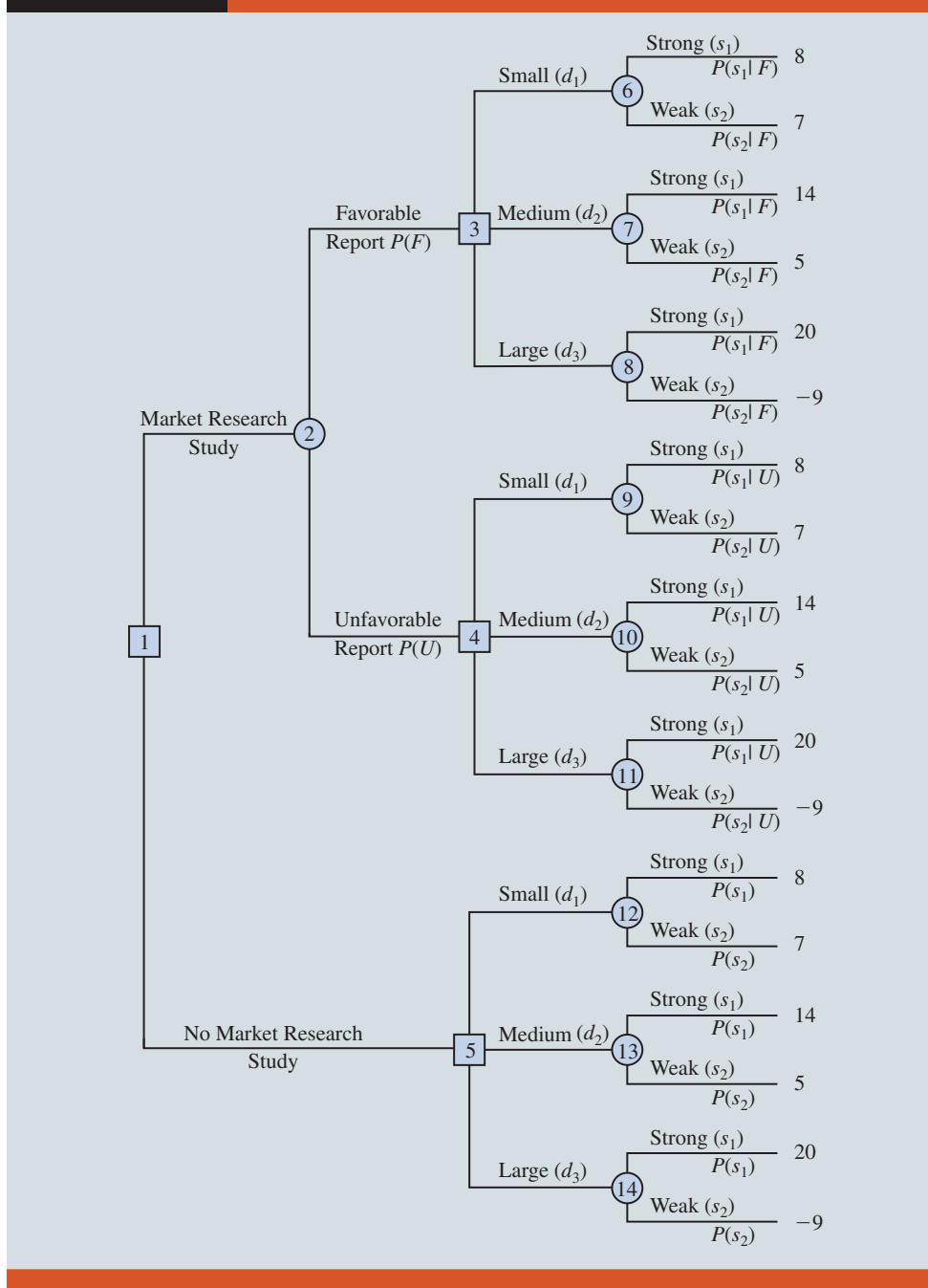
FIGURE 15.10 The PDC Decision Tree
