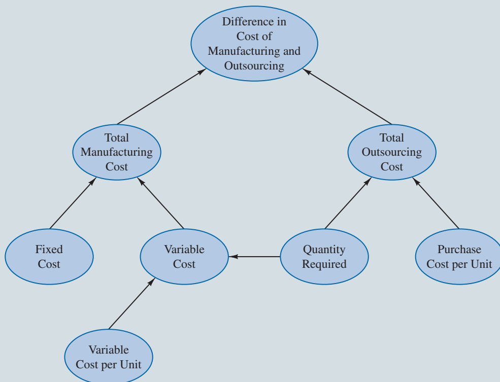
An Influence Diagram for Comparing Manufacturing Versus Outsourcing Cost for Nowlin Plastics
