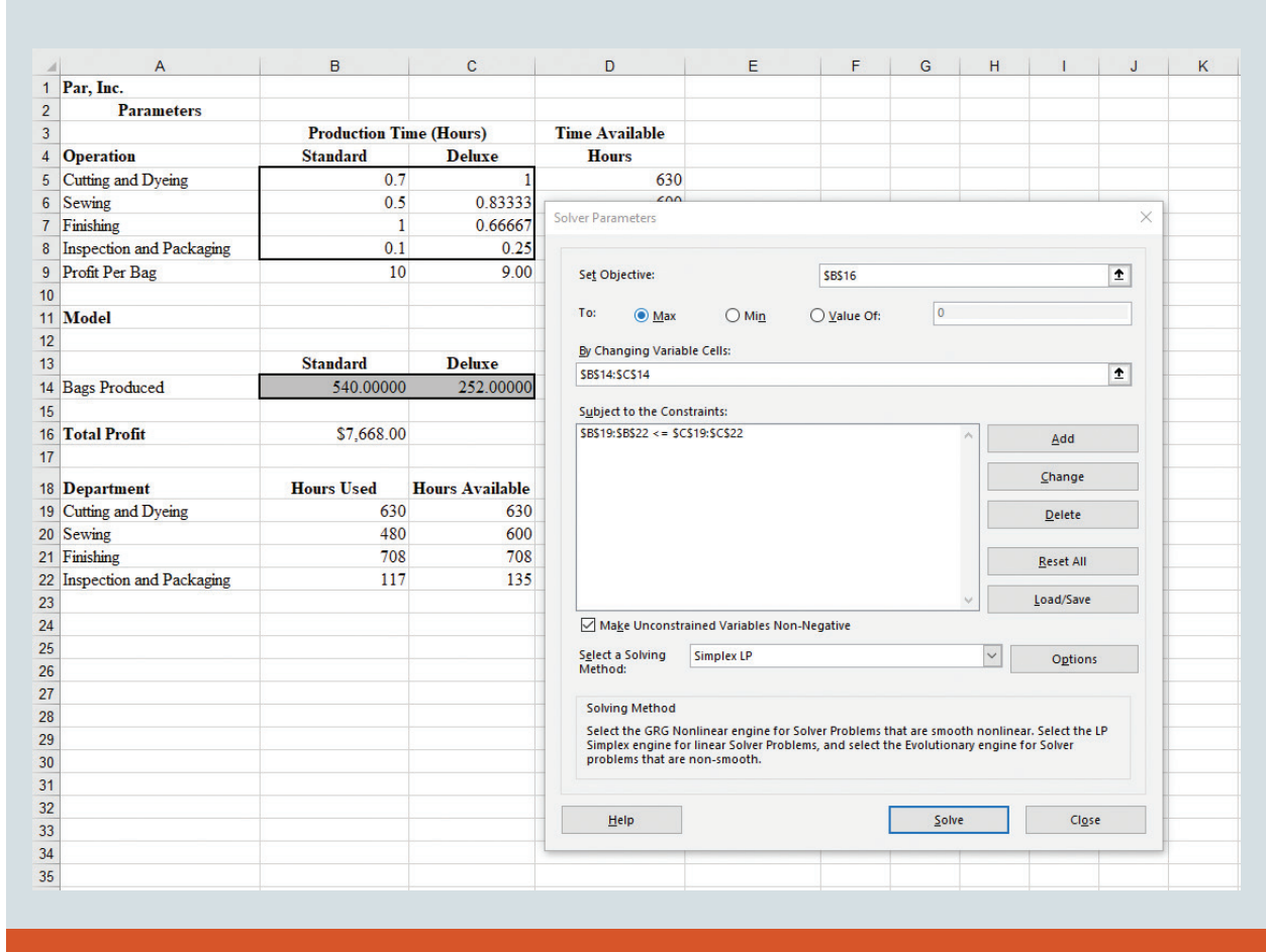
Solver Dialog Box and Solution to the Par, Inc. Problem
