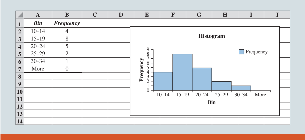
FIGURE 2.14 Completed Histogram for the Audit Time Data Using Data Analysis ToolPak in Excel
