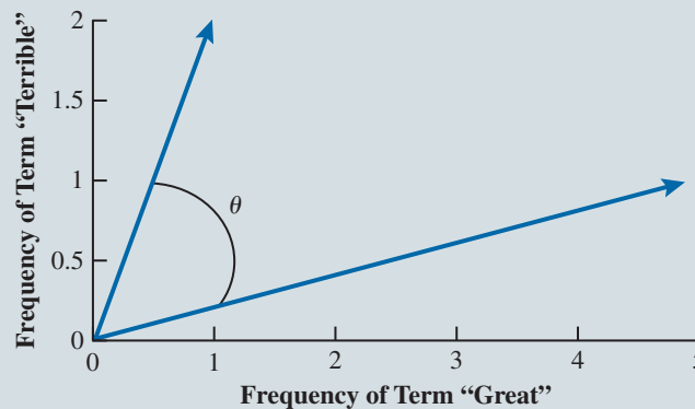
FIGURE 5.9 Visualization of Cosine Distance
