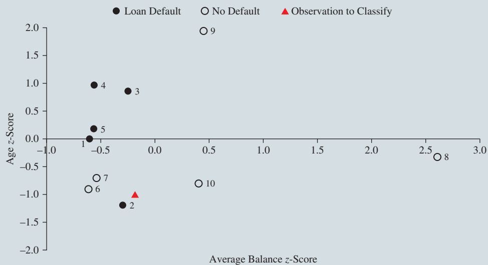
FIGURE 9.7 Scatter Chart for k -NN Classification
