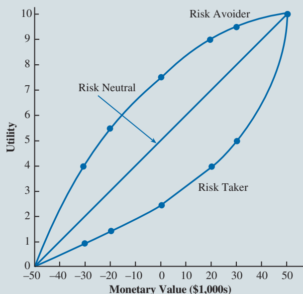
FIGURE 15.11 Utility Function for Money for Risk-Avoider, Risk-Taker, and Risk-Neutral Decision Makers
