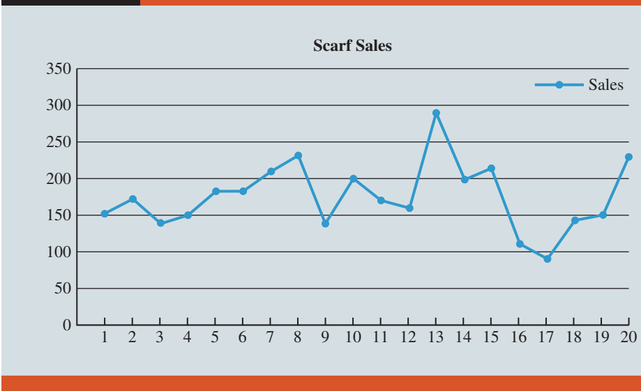
FIGURE 3.3 Example of a Low Data-Ink Ratio Chart
