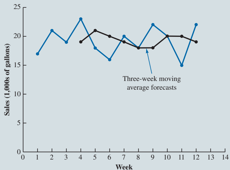
Gasoline Sales Time Series Plot and Three-Week Moving Average Forecasts
