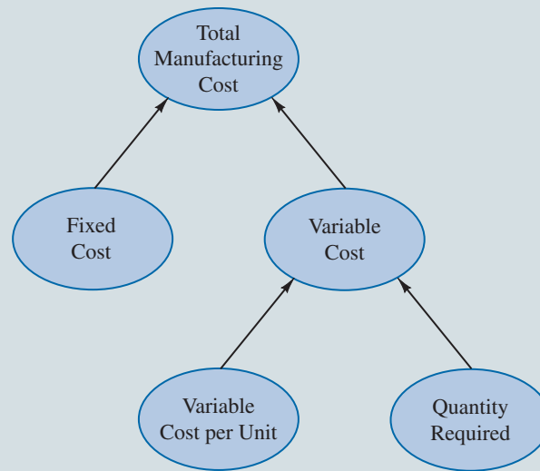
An Influence Diagram for Nowlin's Manufacturing Cost
