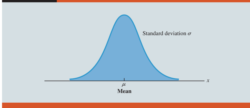
FIGURE 4.21 Bell-Shaped Curve for the Normal Distribution
