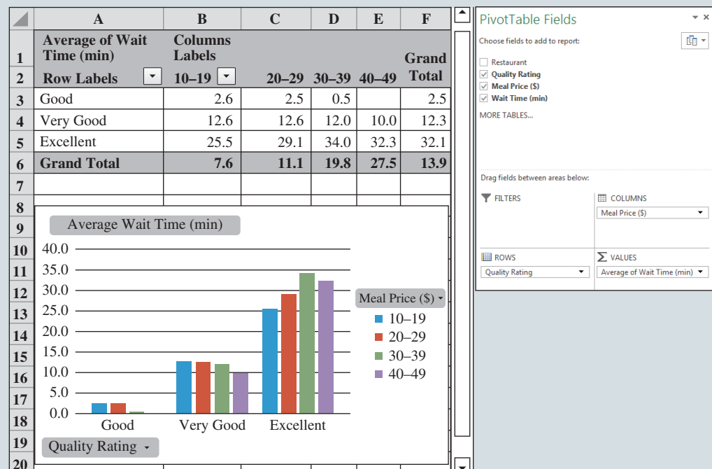
FIGURE 3.32 PivotTable and PivotChart for the Restaurant Data
