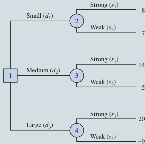
Decision Tree for the PDC Condominium Project ($ Millions)
