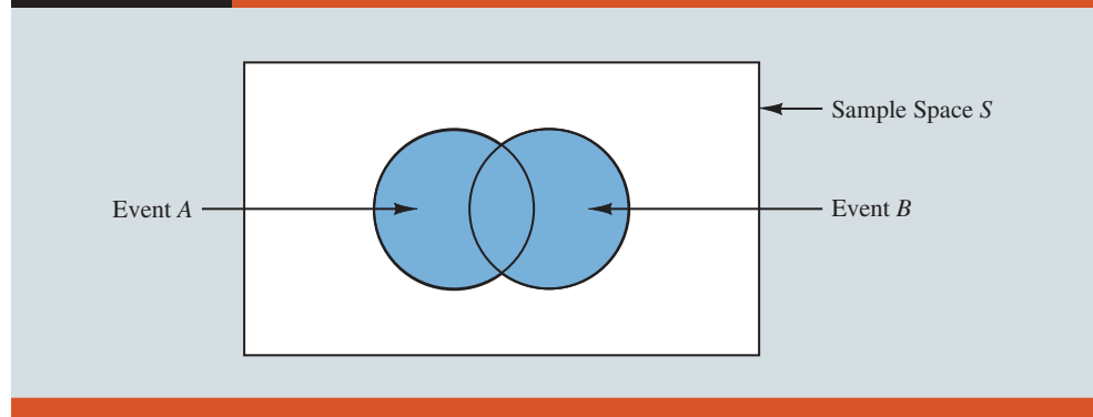
FIGURE 4.2 Venn Diagram for the Union of Events A and B
