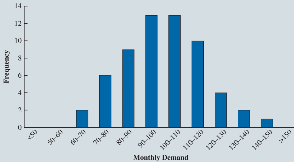
FIGURE 11.12 Distribution of Monthly Router Demand
