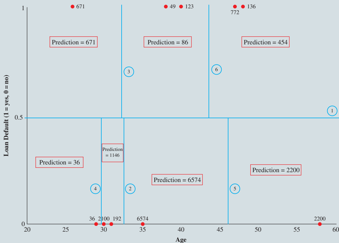
FIGURE 9.13 Geometric Illustration of First Six Rules of a Regression Tree
