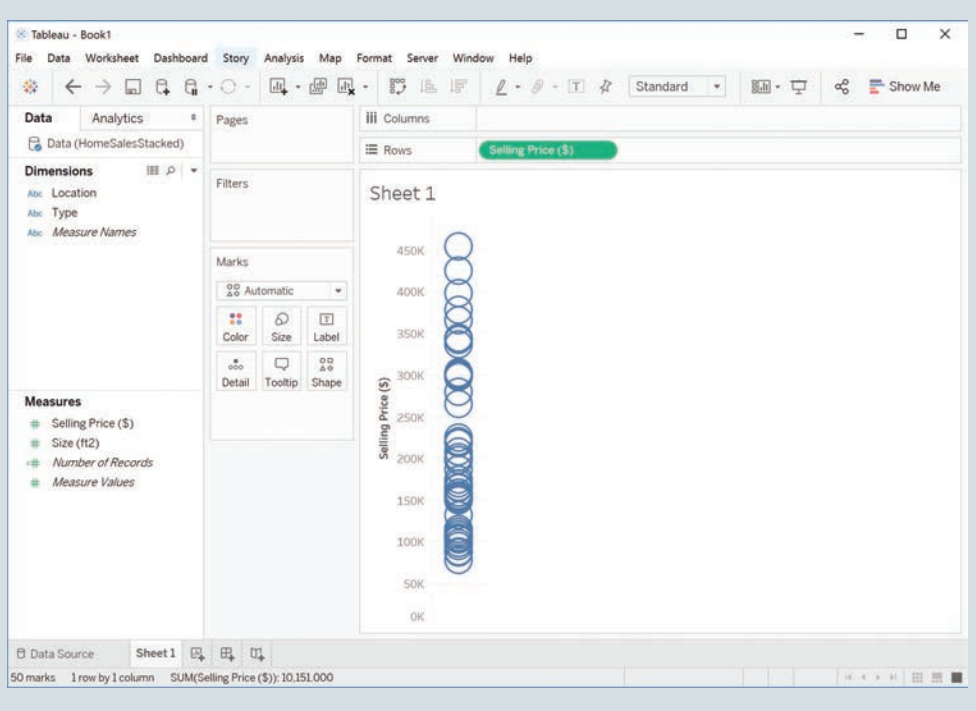
FIGURE TABLEAU 3.19 Disaggregating the HomeSalesStacked Data
