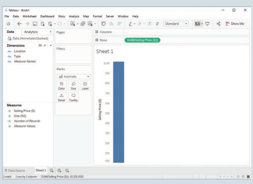
FIGURE TABLEAU 3.18 First Step in Creating a Multiple Variable Boxplot in Tableau for the HomeSalesStacked Data
