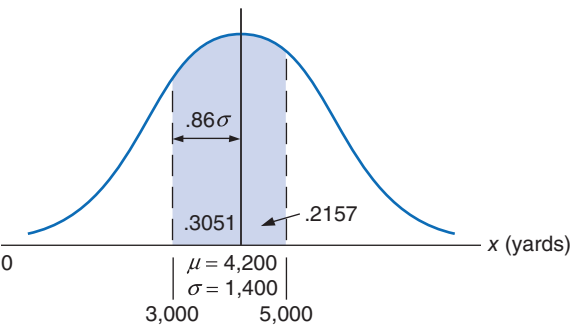
FIGURE 11.13 Normal distribution with P(3,000 \text{ yards} \leq x \leq 5,000 \text{ yards})
