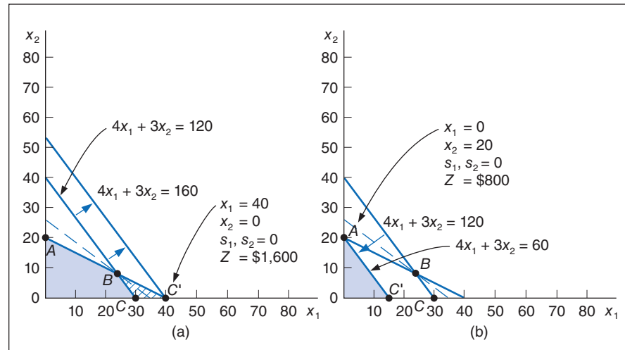
FIGURE 3.8 Determining the sensitivity range for clay quantity
