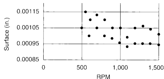
FIGURE 31 Scatter Diagram: Surface Flatness versus Revolutions per Minute
